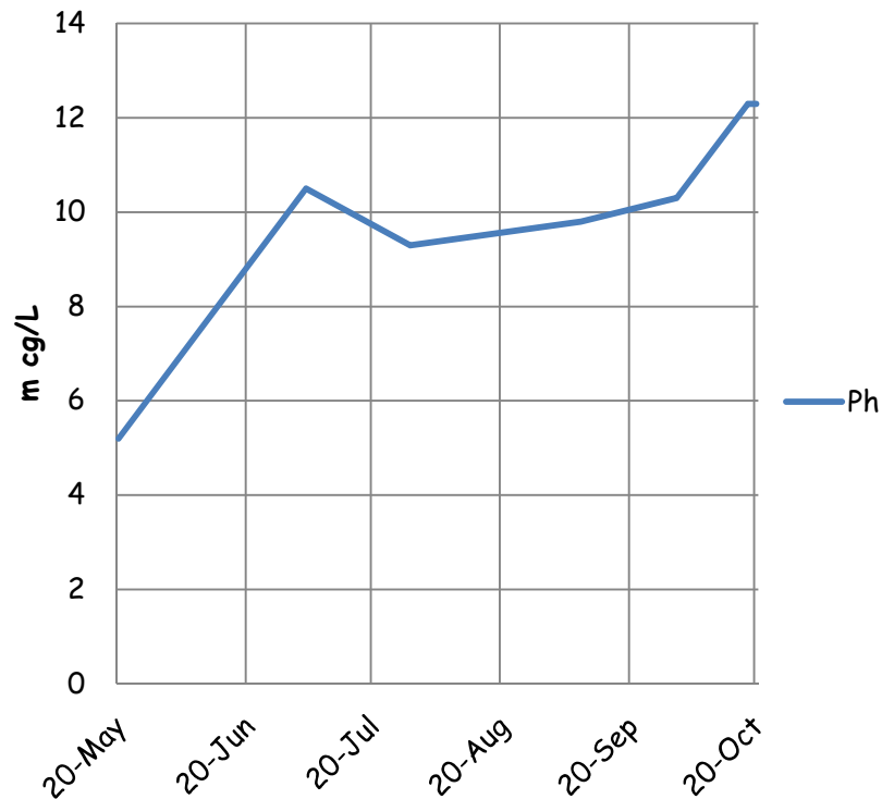
Phosphorus
